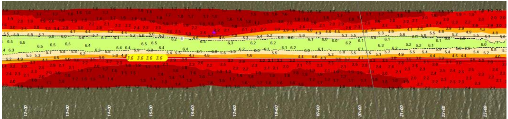
After Dredging Survey – STA 12+00 to 23+00
