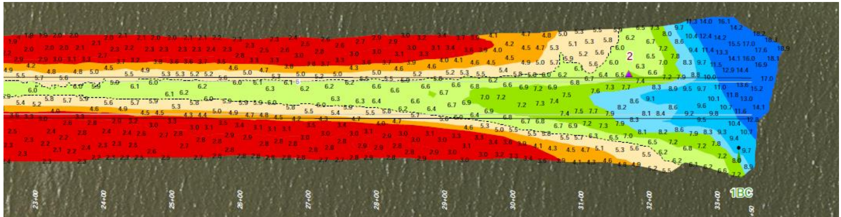
After Dredging Survey – STA 23+00 to 33+50
