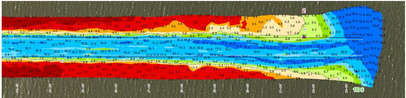
After Dredging Survey – STA 23+00 to 33+50
