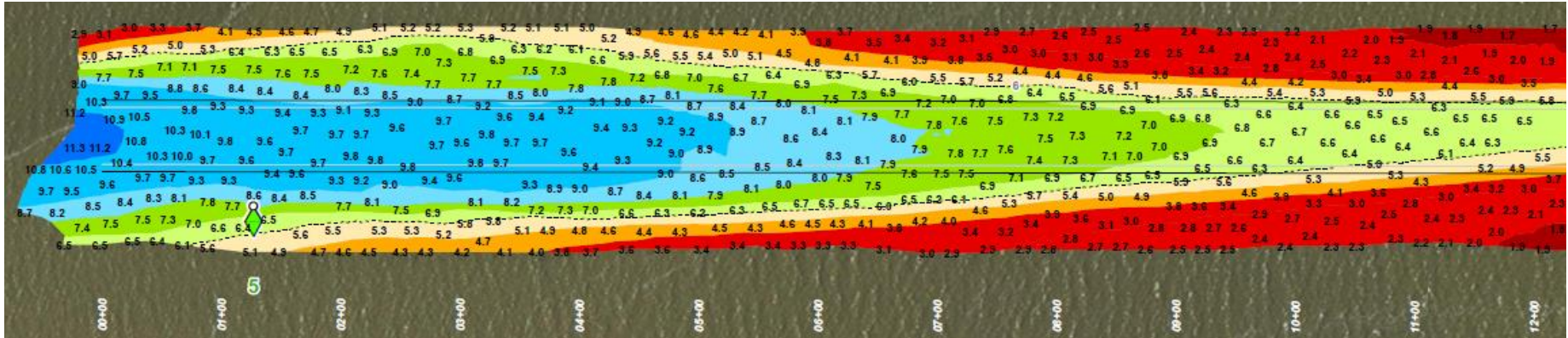
After Dredging Survey – STA 00+00 to 12+00
